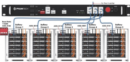
Each battery pile can configure maximum 8pcs US2000B Plus or 8 pcs US3000
